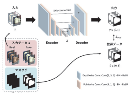
(2+1)D CNNを用いた手法 [2]
