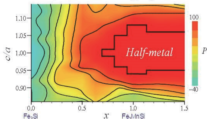
Spin polarization of \text{Fe}_{3-x}\text{Mn}_x\text{Si}
